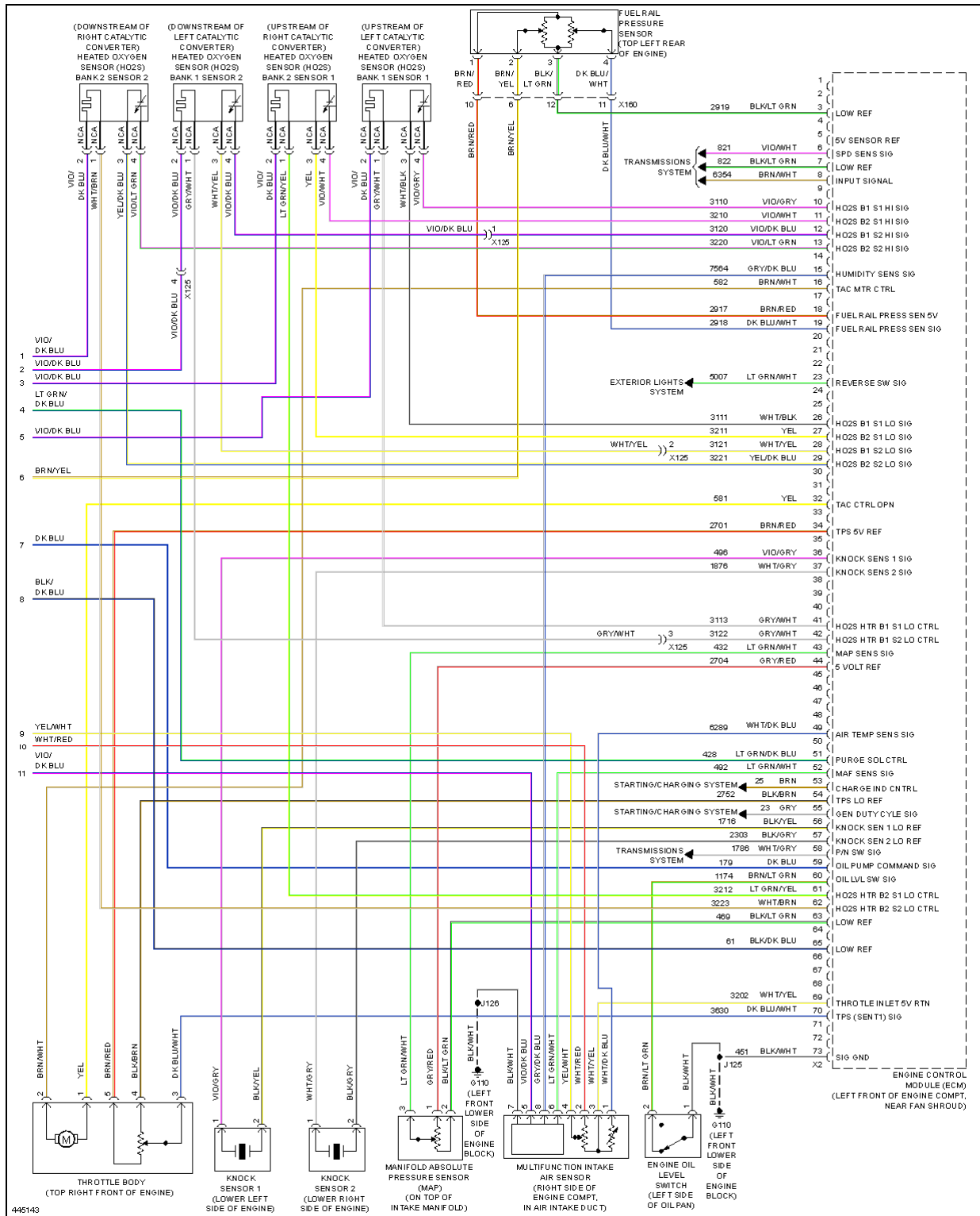
Fig. 43: 6.2L VIN J, Engine Performance Circuit (6 of 6)
