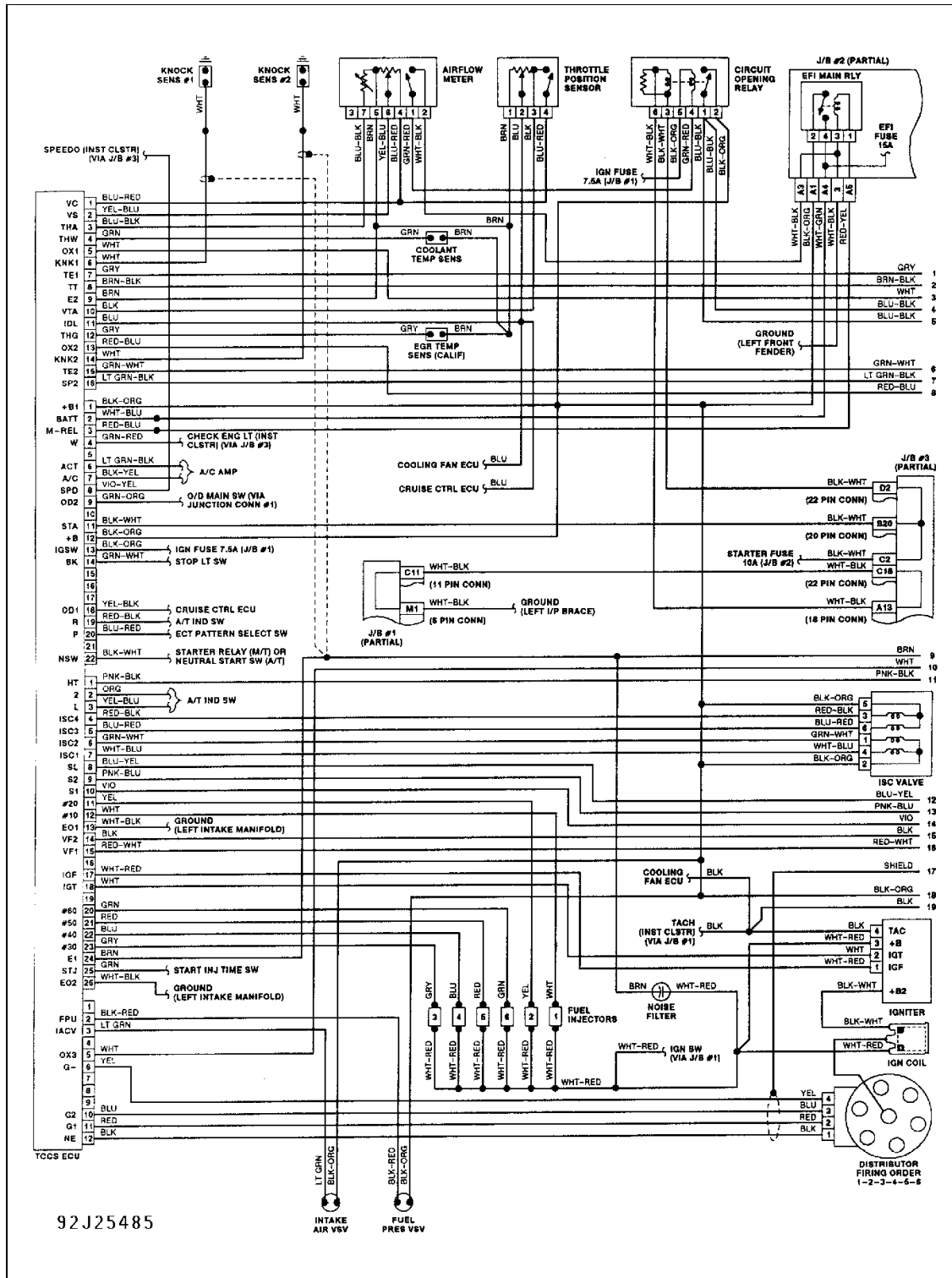
Fig 3: Wiring Diagram (Camry 3.0L - 1 of 2)
