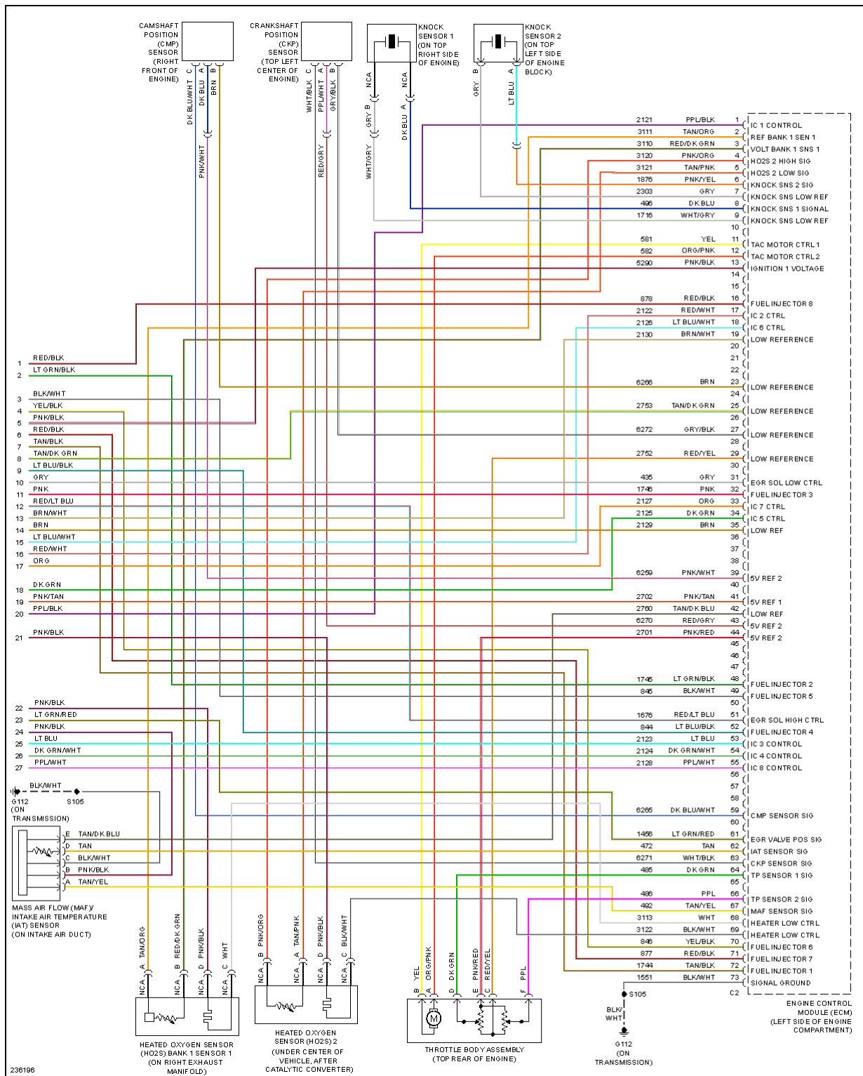
Fig. 27: 4.6L VIN 9, Engine Performance Circuit (5 of 5)
