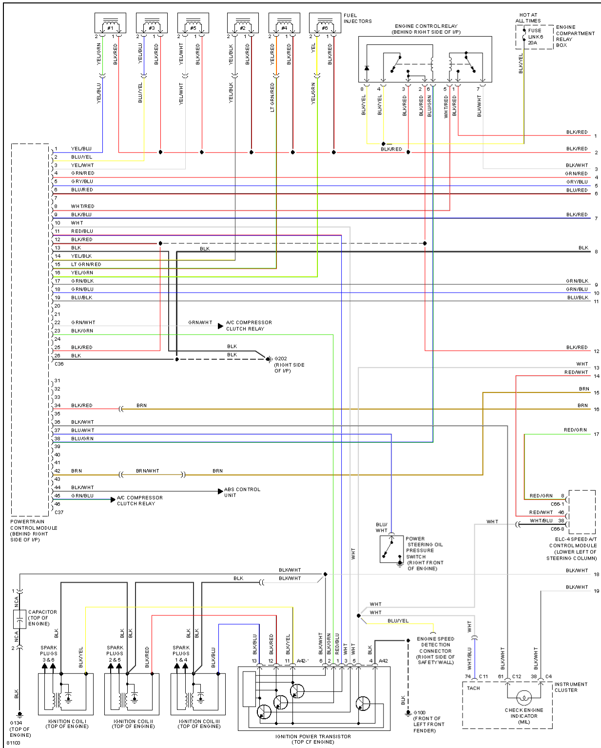
Fig. 16: 3.0L 24 Valve, Engine Performance Circuits, Federal (1 of 3)
