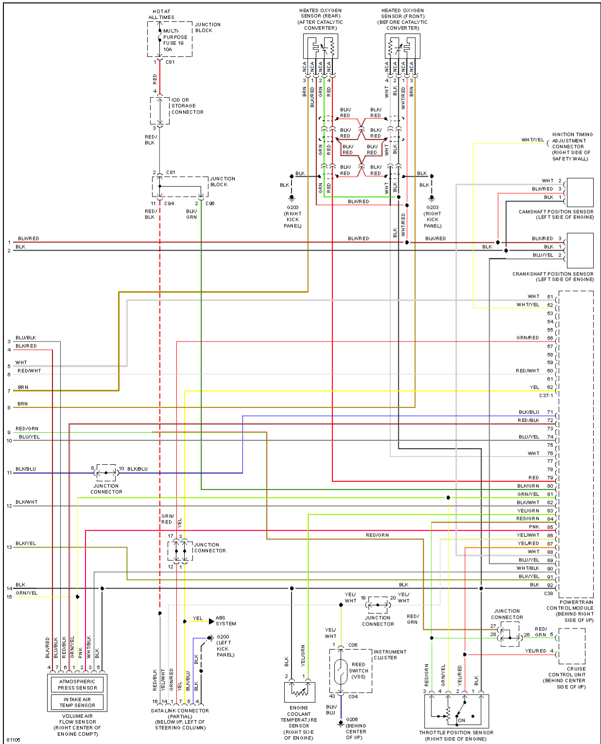
Fig. 18: 3.0L 24 Valve, Engine Performance Circuits, Federal (3 of 3)
