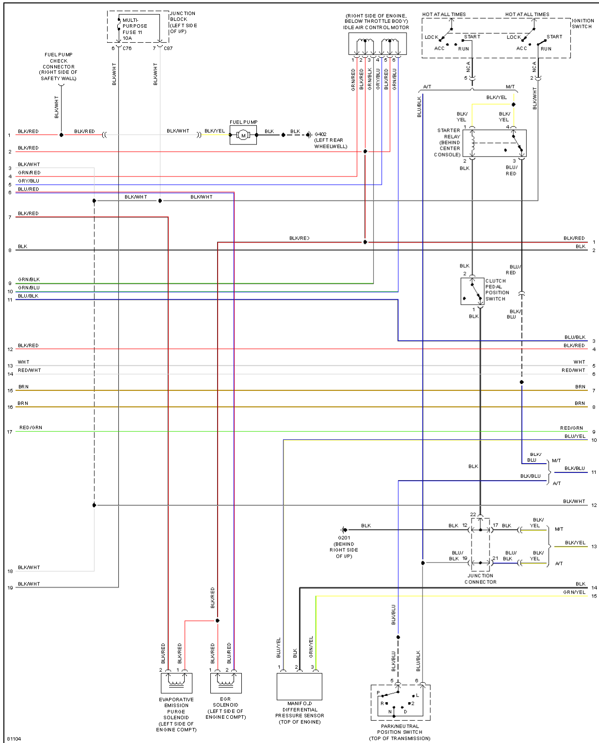
Fig. 17: 3.0L 24 Valve, Engine Performance Circuits, Federal (2 of 3)
